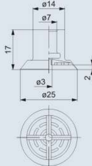
ZP3P-25PTSF 净重：2.2g
