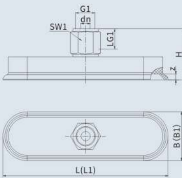
•MAOF50x16~120x60 (内螺纹)
