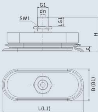
•MAOB60x30~110x55 (外螺纹)
