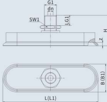
•MAOF50x16~120x60 (外螺纹)
