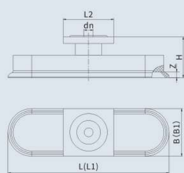
•MAOF50x16~120x60RA (矩形适配器)
