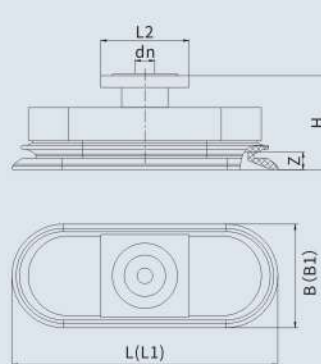
•MAOB60x30~110x55RA (矩形适配器)
